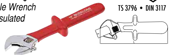
Krom vanadyum, Krom kaplı, Kalın PVC izoleli Chrom vanadium, Chrom plated, Double PVC insulated
